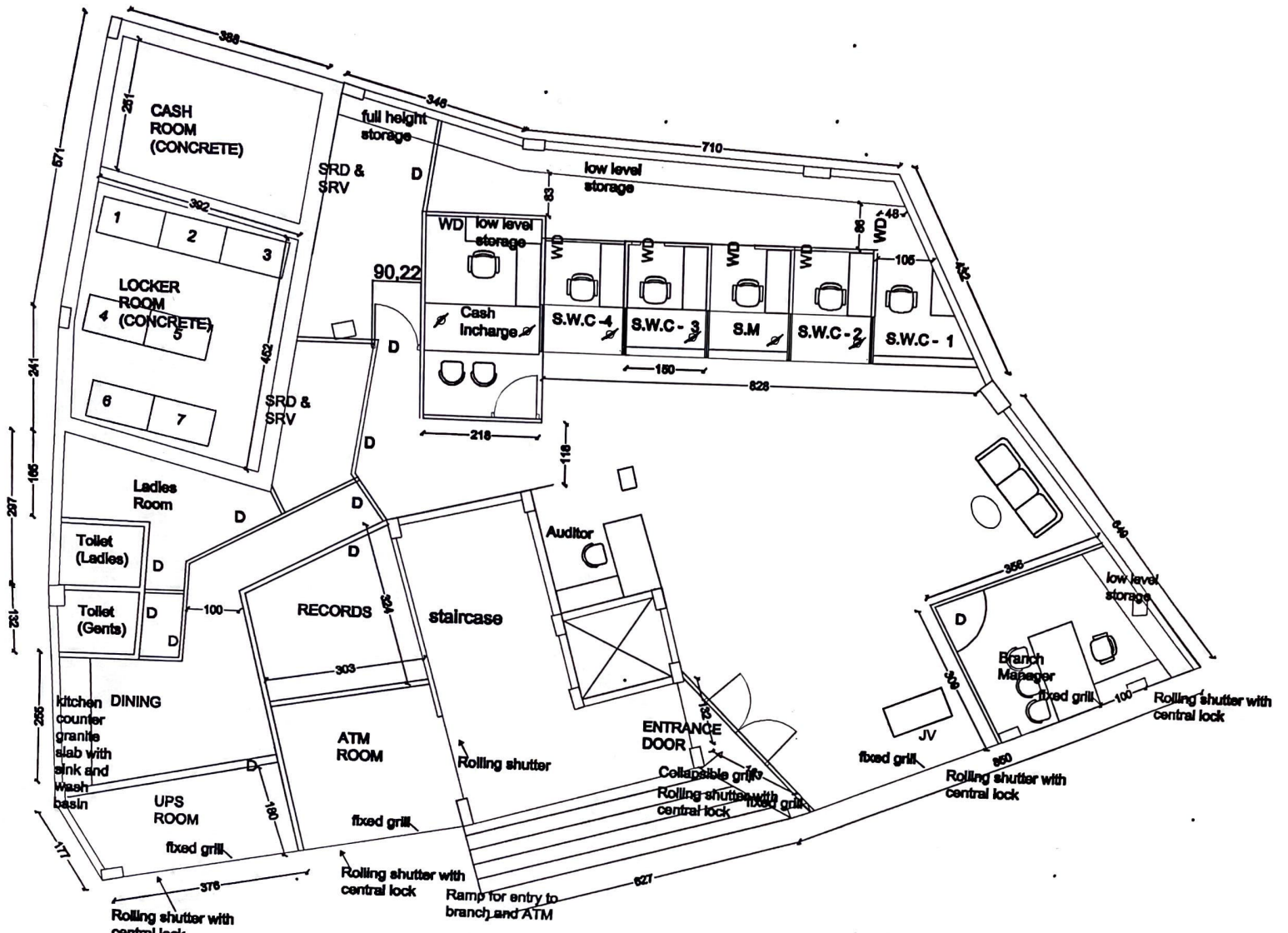
SBI AMBALAMUKKU-GROUND FLOOR- DWG NO.2 DT. 24.09.24
